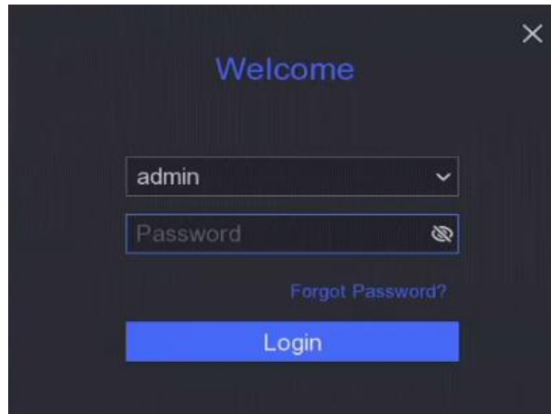
Figure 1-4 Login Interface
