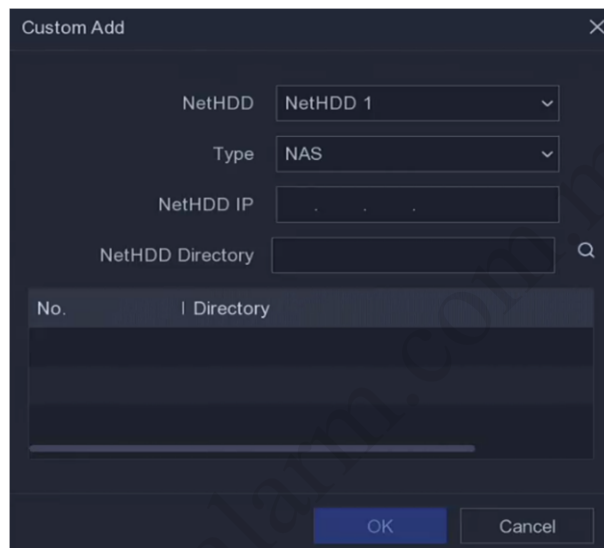
Figure 6-26 Add NetHDD
