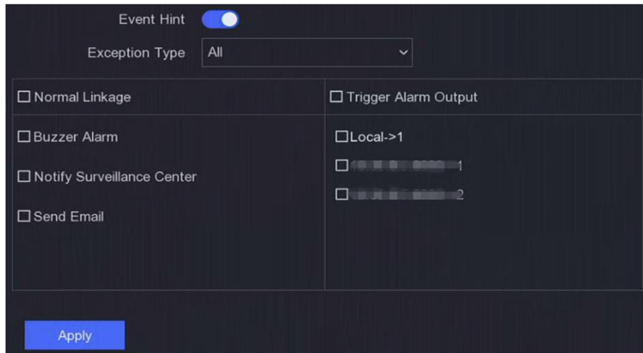
Figure 5-3 Exceptions
