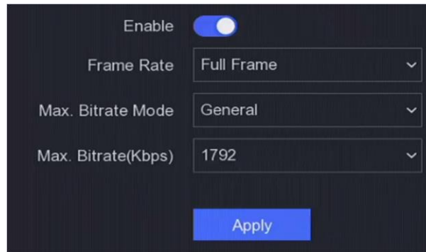
Figure 6-5 Channel-Zero
