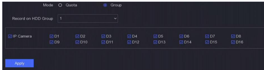
Figure 6-27 Group
