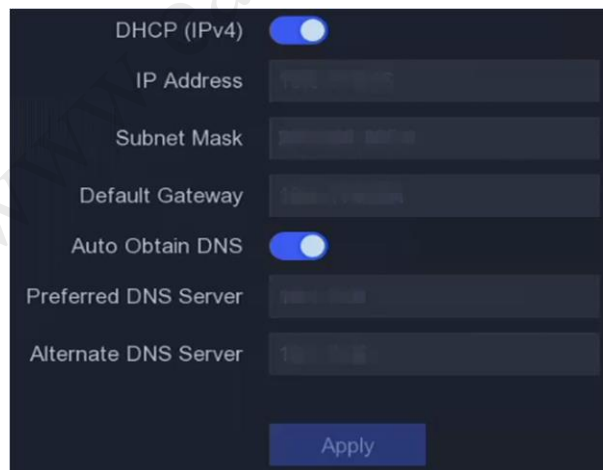
Figure 5-4 Network
