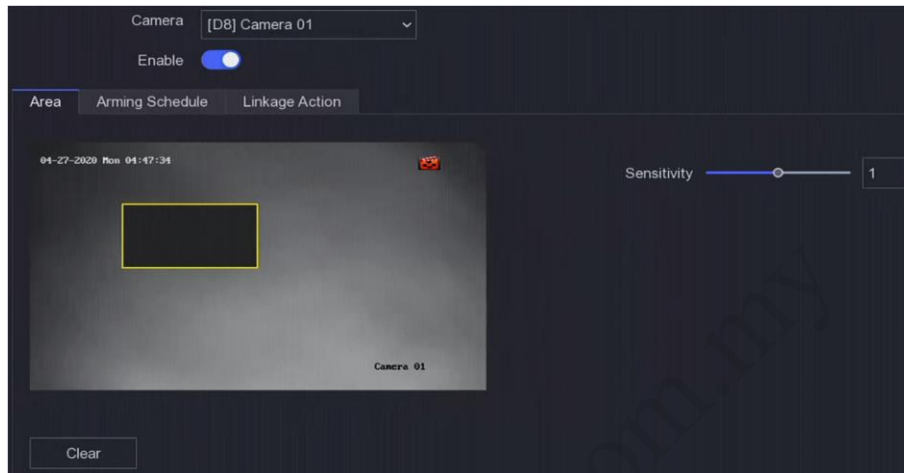
Figure 6-16 Video Tampering
