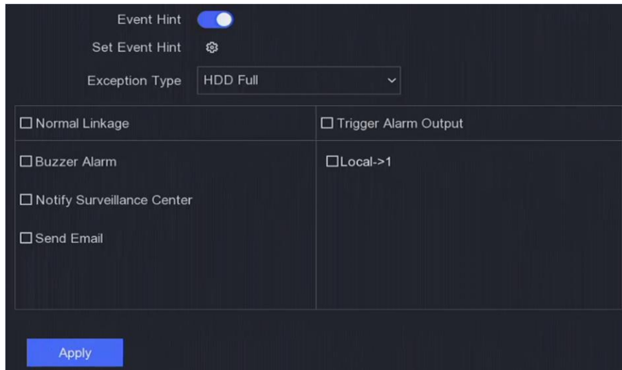
Figure 6-21 Exceptions
