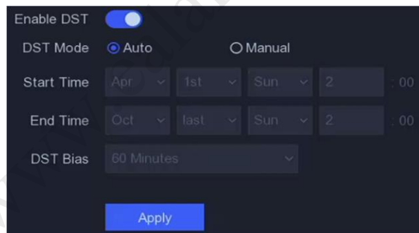
Figure 6-2 DST Settings
