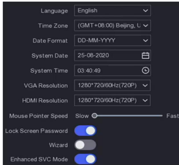
Figure 6-1 Basic Settings
