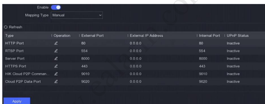
Figure 6-7 NAT
