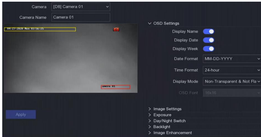
Figure 6-14 OSD
