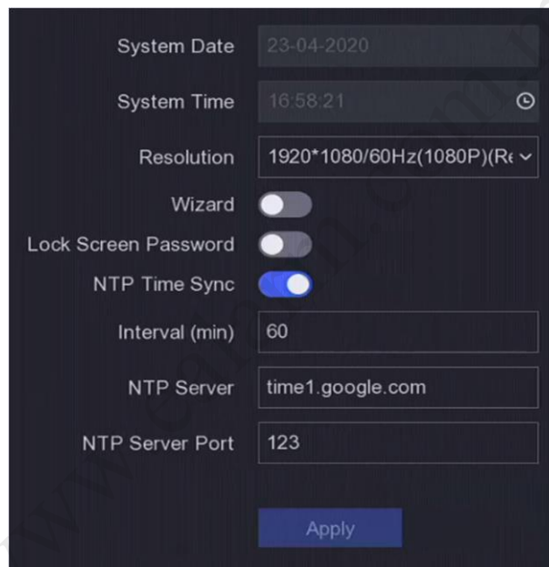
Figure 5-1 General Settings
