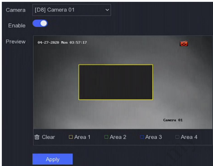
Figure 6-15 Privacy Mask
