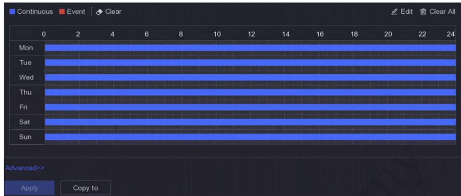
Figure 6-24 Recording Schedule
