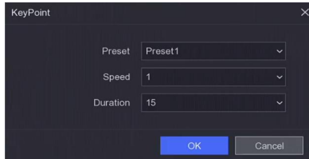
Figure 2-3 Patrol Settings
