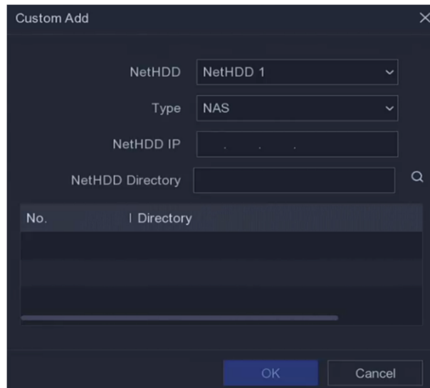
Figure 5-17 Add NetHDD
