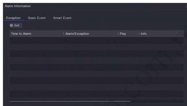
Figure 8-1 Alarm Center
